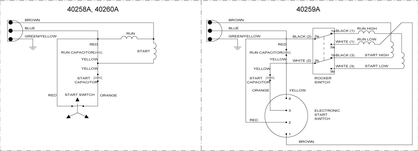
MOTOR DIAGRAM
